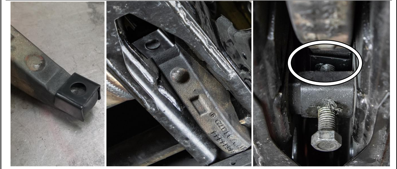
Figure 62: Cognito Torsion Key Retainer
