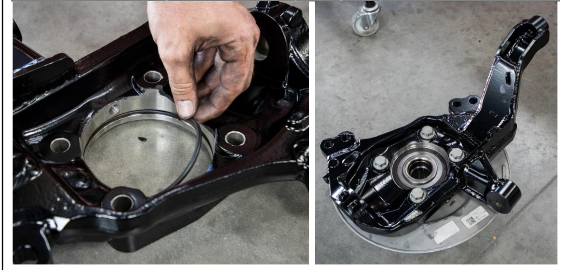
Figure 49: Hub Assembly on Cognito Spindle
