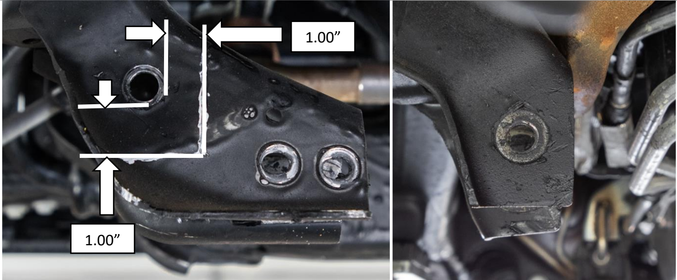
Figure 25: Trim Rear Crossmember
