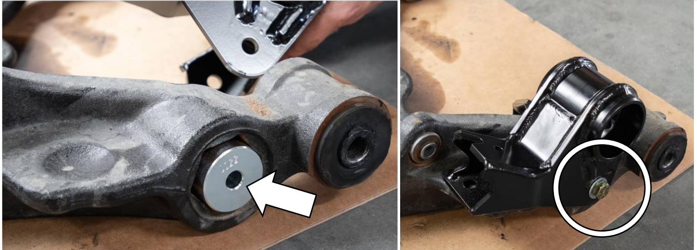
Figure 42: Install Non Torsion Bar Drop Bracket
