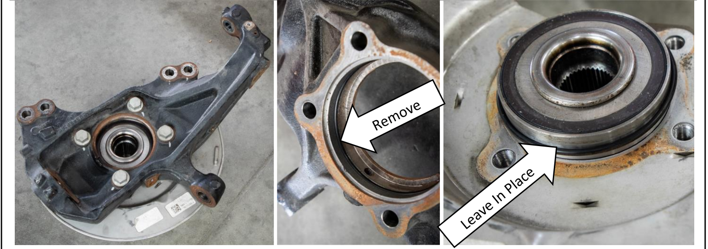
Figure 48: Disassemble Hub Assembly
