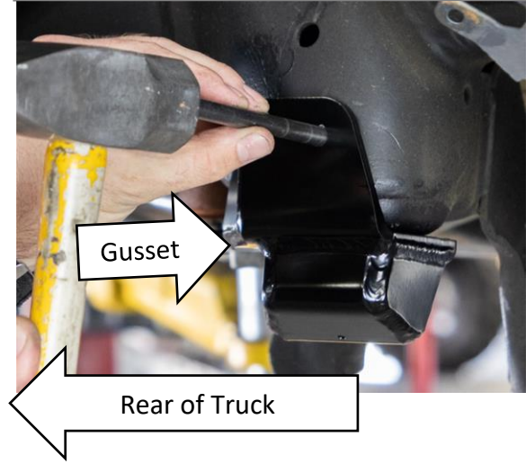
Figure 35: Drill Bump Stop Mounting
