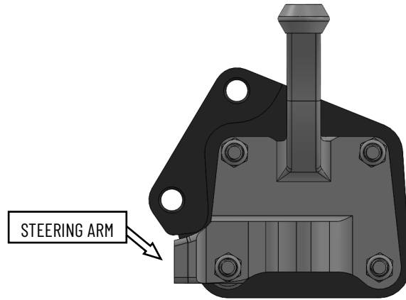
Figure 3. Base bracket installed (inboard view)
