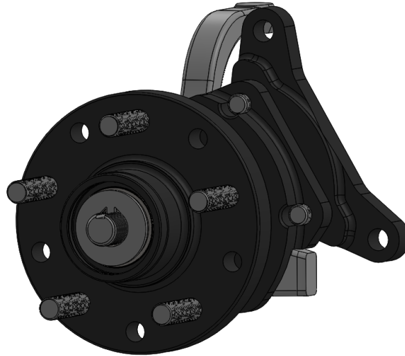
Figure 5. Wheel hub assembly installed
