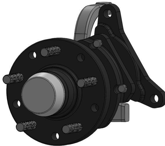
Figure 6. Cotter pin and dust cap installed (right passenger side shown)
