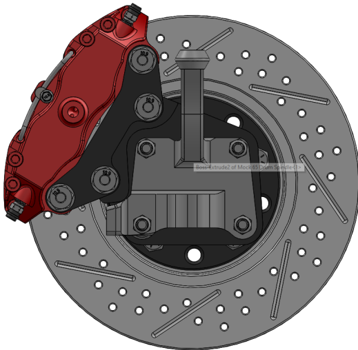
Figure 8. Caliper assembly installed inboard view (left driver side shown)
