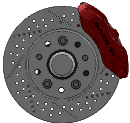
Figure 9. Caliper assembly installed outboard view (left driver side shown)
