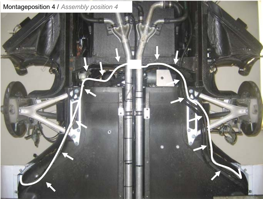
Montageposition 4 / Assembly position 4
