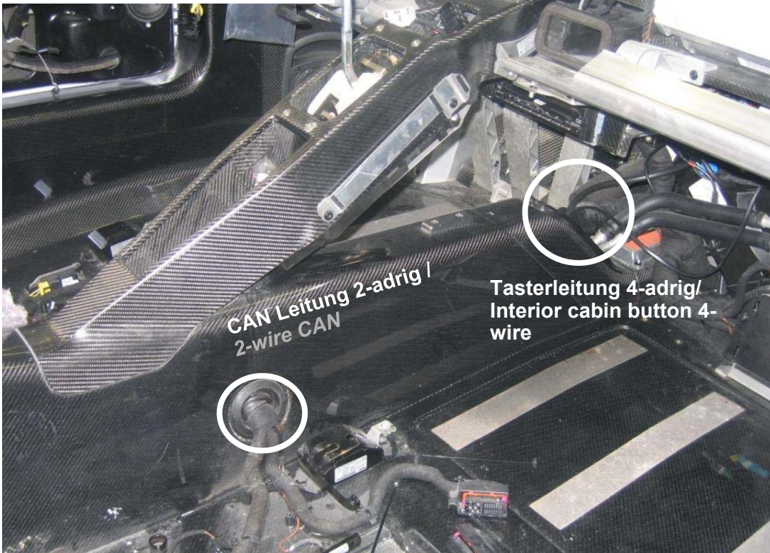
Montageposition 7, 8 / Assembly position 7, 8
