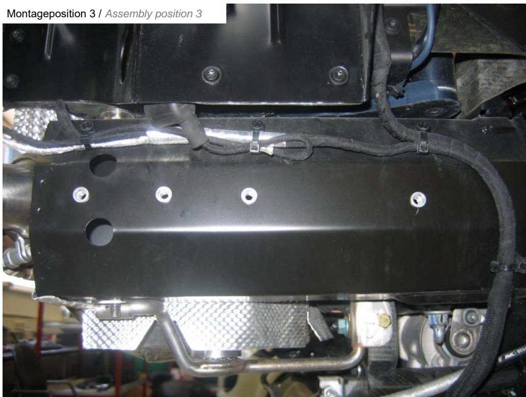
Montageposition 3 / Assembly position 3
