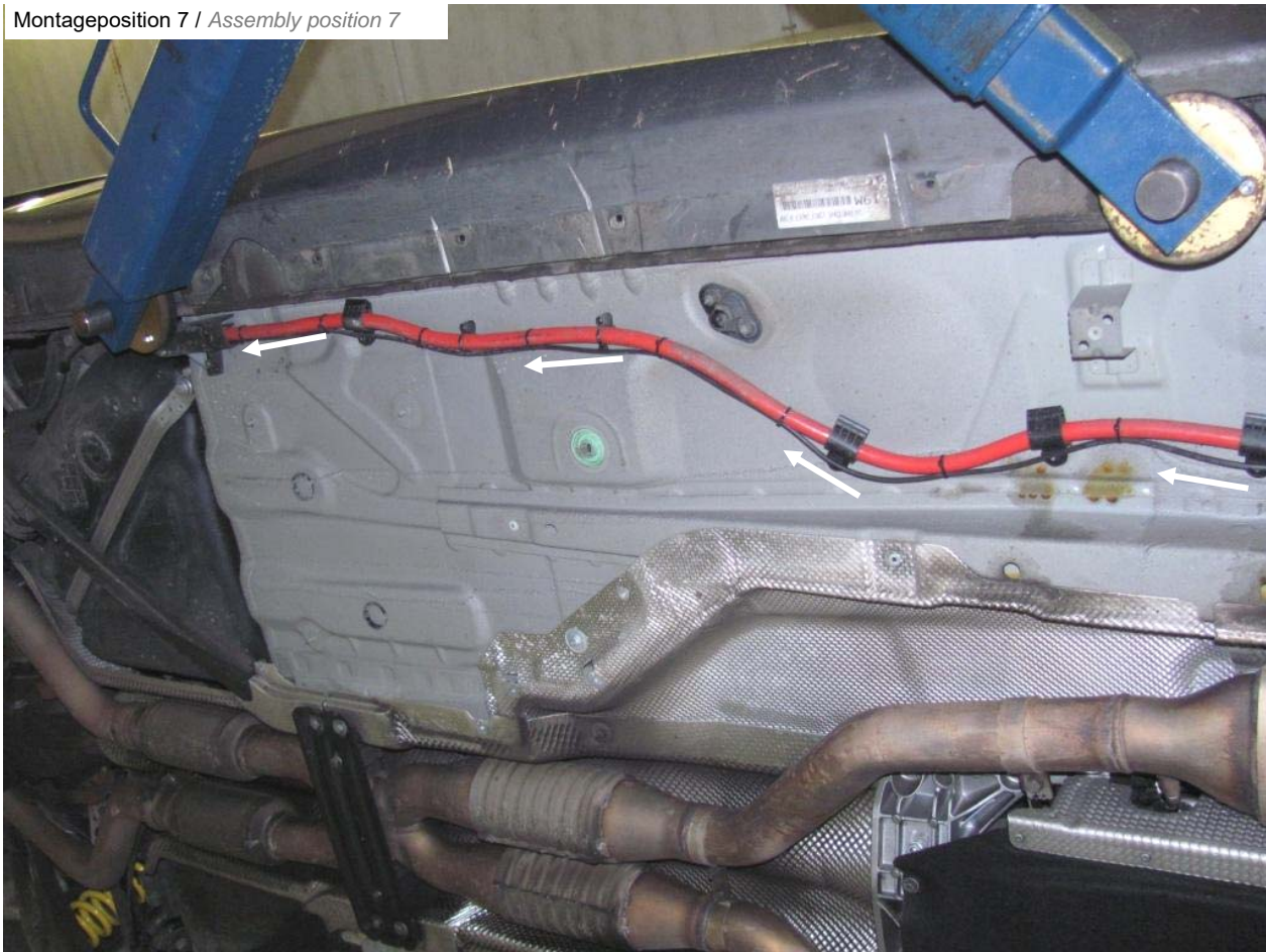
Montageposition 7 / Assembly position 7
