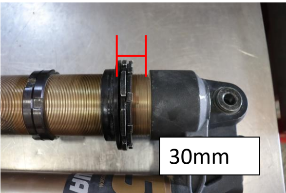
Step 11. Set pre-load spring seat to 30mm (1 3/16in.) from bottom of seat to bottom of reservoir bridge.
