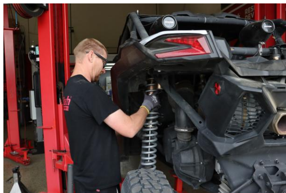
Step 18. Set shock assembly in vehicle by inserting top of assembly through opening in body panels and setting lower shock mount in trailing arm.
