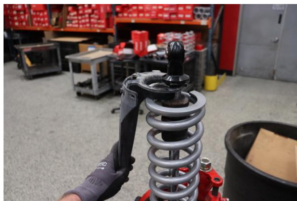
Step 16. Install lower spring retainer. Decompress spring assembly making sure that lower spring retainer and main spring sit flush with lower shock mount.
