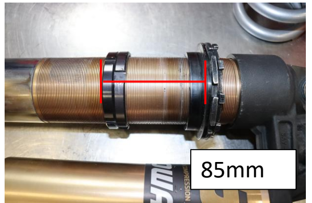
Step 12. Set crossover ring to 85mm (3 3/8in.) from bottom of spring seat to bottom of crossover ring.
