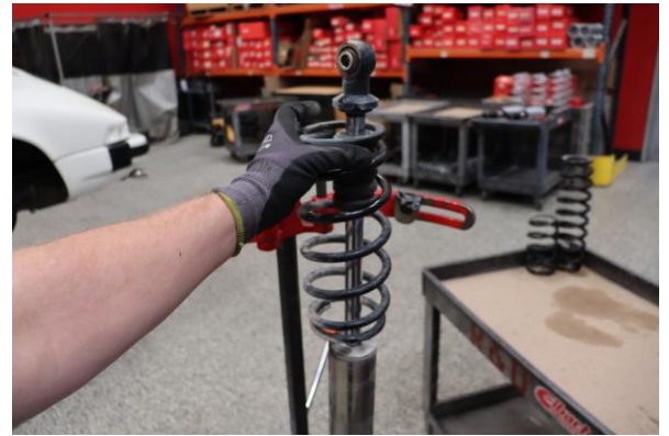
Step 10. Remove OE secondary spring.
