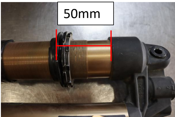
Step 11. Set pre-load to 50mm ( 2in.) from bottom of spring seat to bottom of furthest point on reservoir bridge.
