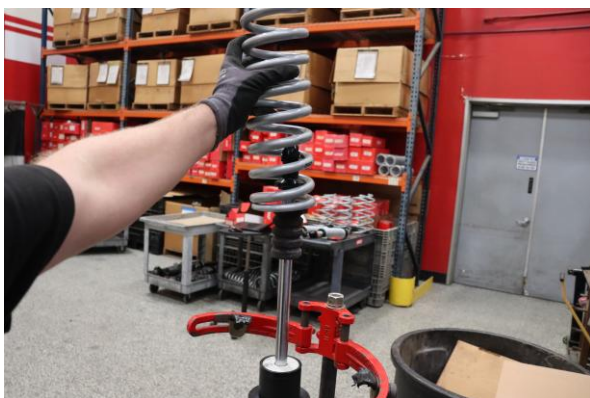
Step 15. Install Eibach rear main spring.
