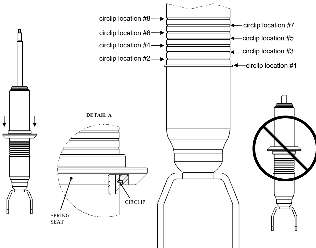
B8 6112 Typical Lift Heights**
