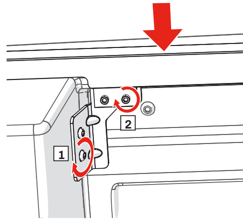
Tailgate Hardware
