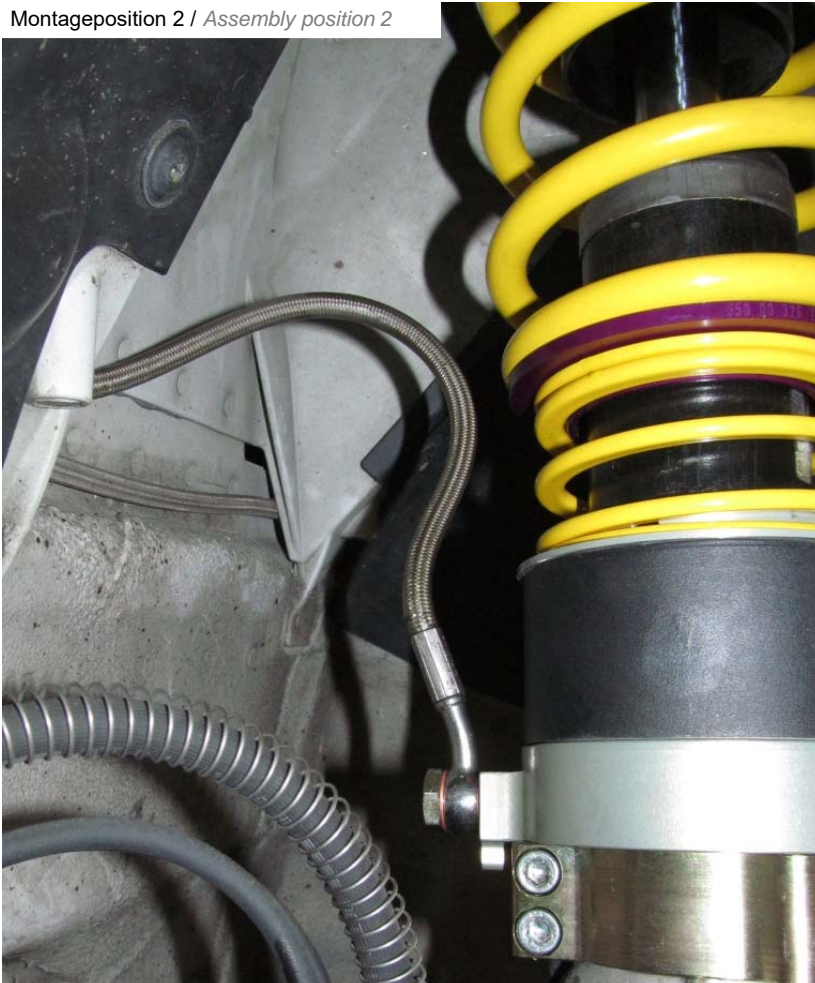
Montageposition 2 / Assembly position 2
