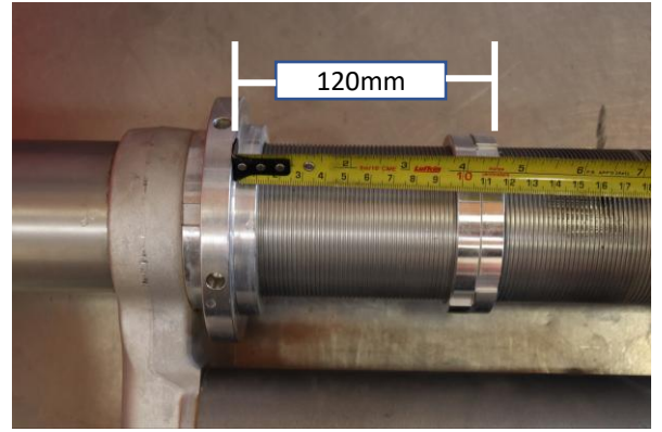
Set the preload collar all the way up to the Resi bridge and the crossover ring to 120mm (4 47/64") from the spring seat to the bottom of the crossover ring.
