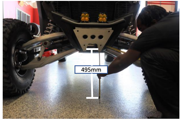
The front height should measure about 495mm (19 31/64") from the ground to the lower control arm bolt.
