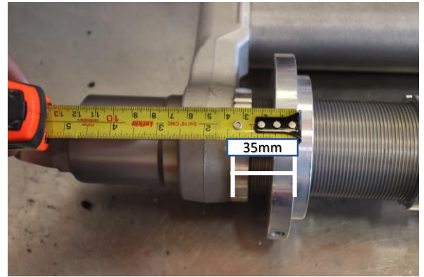
Set the preload collar to 35mm (1 3/8") from the bottom of the Resi crossover to the bottom of the preload collar
