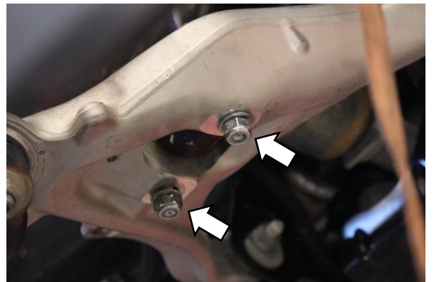
18. Tighten the nuts for the lower shock mount with a 19mm wrench
