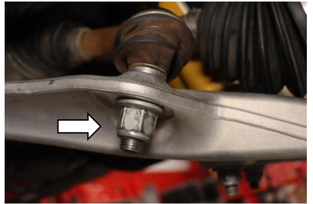
22. Install the sway bar end link and secure the nut using an 18mm socket.
