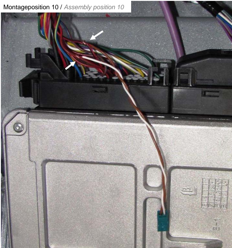
Montageposition 10 / Assembly position 10
