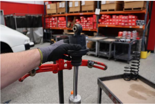
Step 9. Remove OE spring slider.
