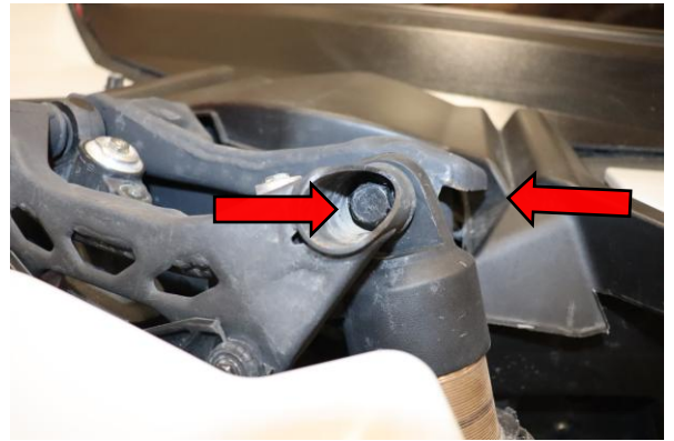
Step 4. Remove 18mm upper shock bolt and nut from both left and right front. Need socket and wrench.
