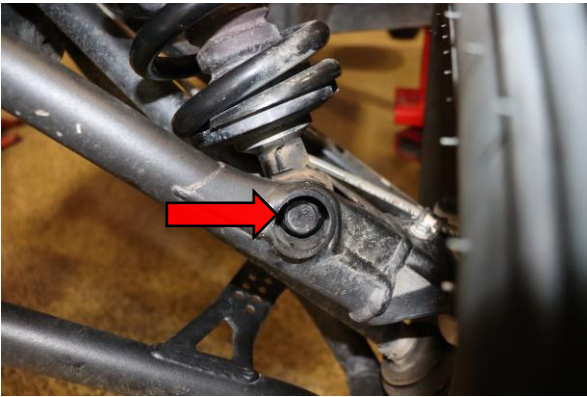
Step 3. Remove 18mm lower shock nut and bolt. Need 2 18mm sockets
