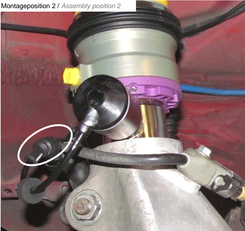
Montageposition 2 / Assembly position 2
