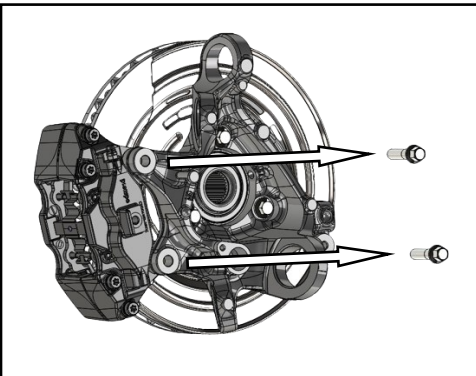
FIGURE 1. REMOVAL OF CALIPER MOUNTING HARDWARE
