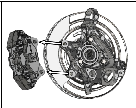
FIGURE 2. REMOVAL OF CALIPER FROM KNUCKLE (BRAKE HOSE NOT SHOWN IN PHOTO)
