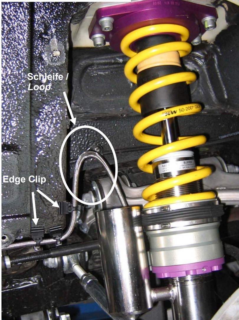
Montageposition 10 / Assembly position 10
