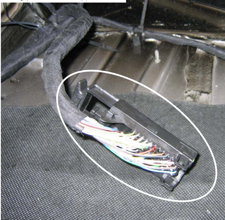
Montageposition 8 / Assembly position 8
