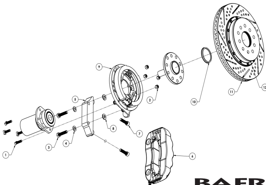
Figure 1. Exploded Isometric View of Pro+ Installation Configuration
