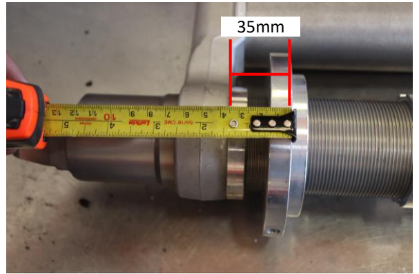
Set the preload collar to 35mm (about 1 3/8") from the bottom of the Resi crossover to the bottom of the preload collar
