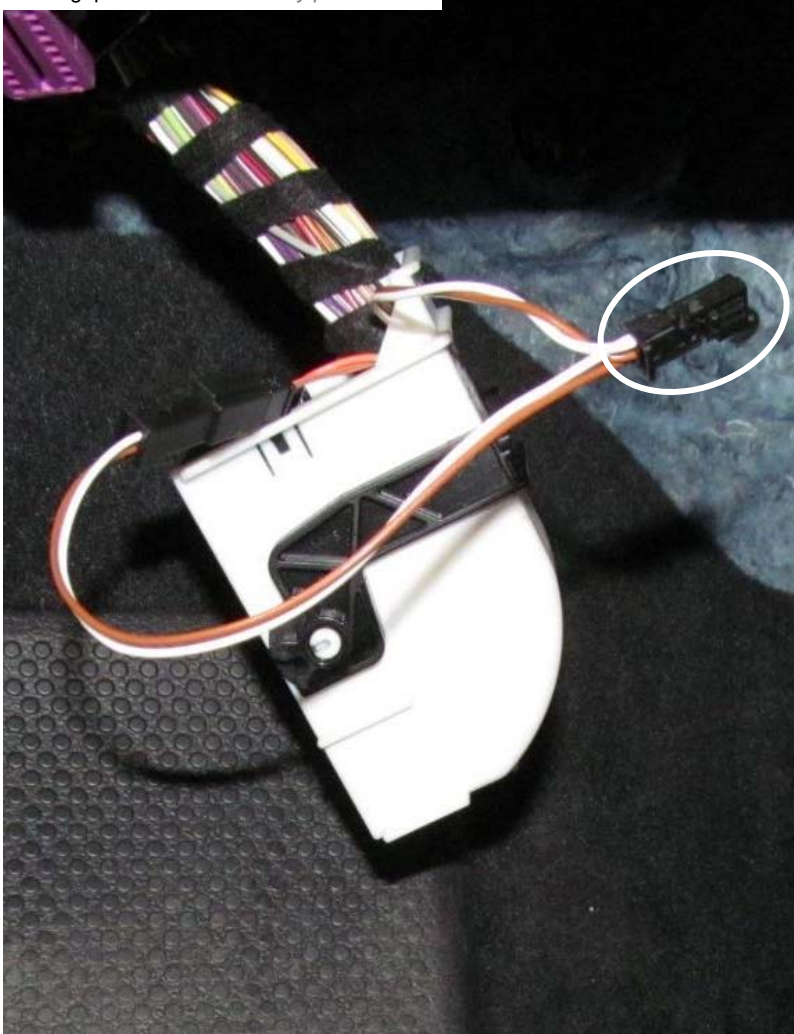
Montageposition 11 / Assembly position 11
