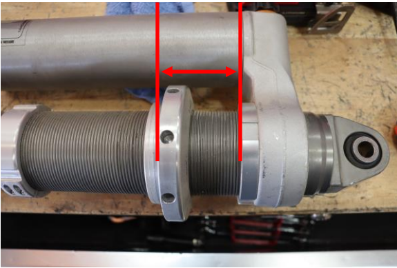
Step 15. Set pre-load to 65mm (2 1/2in.) from bottom of spring seat to bottom of reservoir bridge collar.
