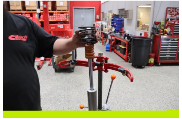
Step 14. Remove the second OE tender spring.
