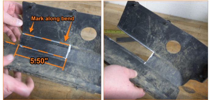
19. Trim the back of the grille support as shown in the below images.
