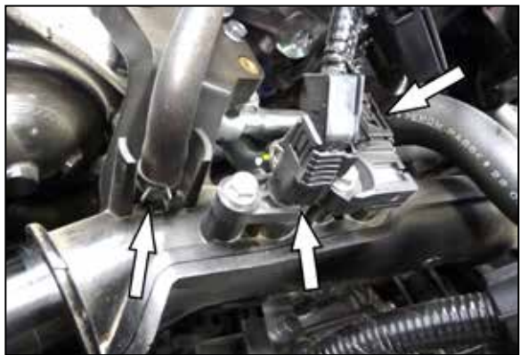
7. Disconnect the two pressure sensor electrical connections. Disconnect the vacuum hose from the upper charge tube.
