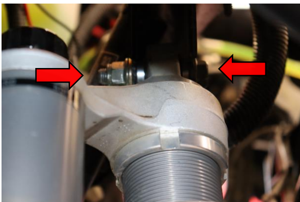
Step 5. Remove the upper shock hardware 15mm socket and wrench.
