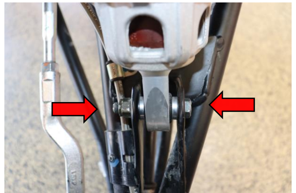
Step 4. Remove lower shock mount nut using 15mm socket and wrench.
