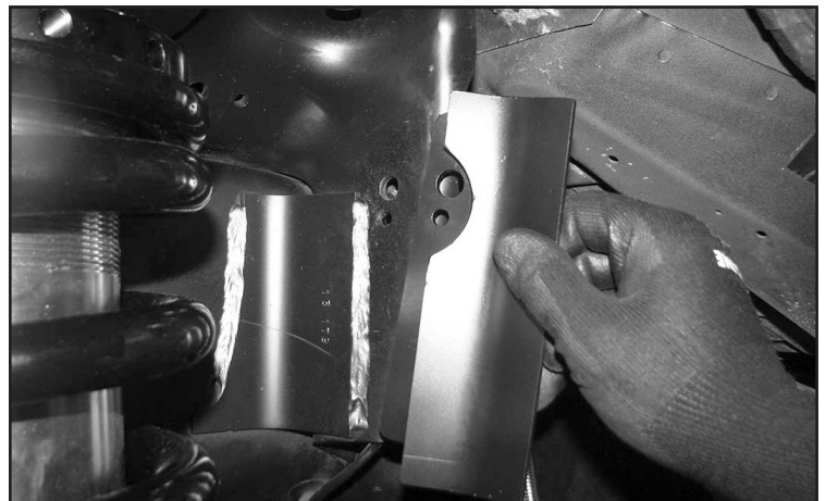
FIGURE 38 - STEP 24
