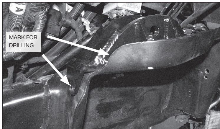
FIGURE 6 - STEP 5
