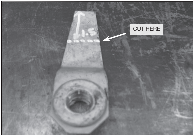
FIGURE 41 - STEP 27
