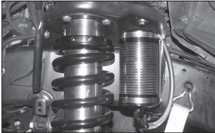
FIGURE 40 - STEP 25
