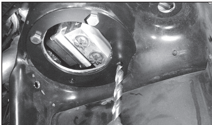
FIGURE 9 - STEP 6
