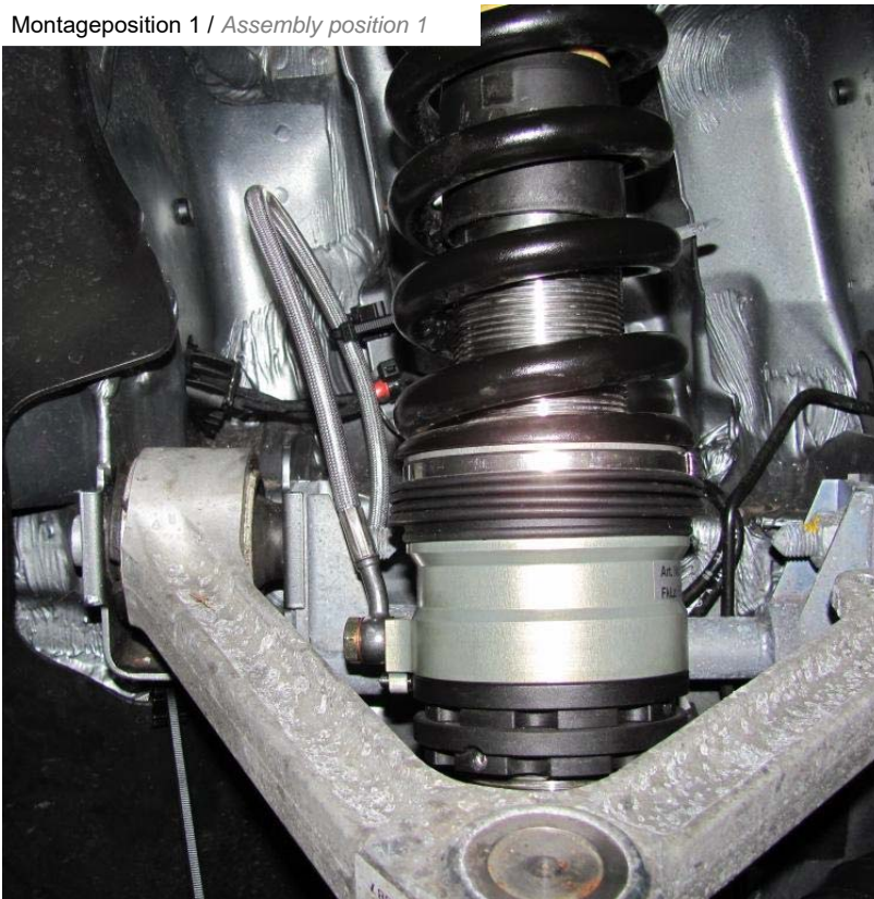
Montageposition 1 / Assembly position 1
