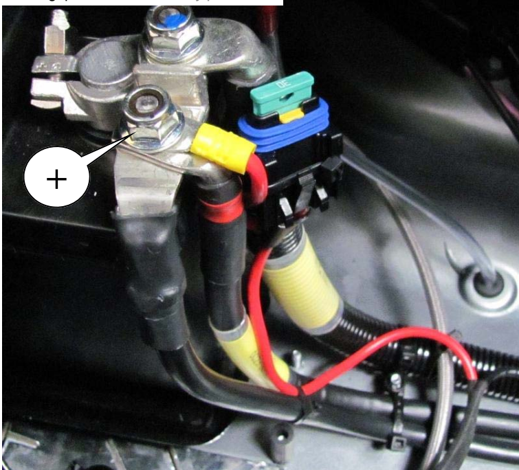
Montageposition 3 / Assembly position 3
