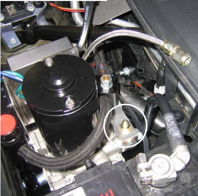
Montageposition 3 / Assembly position 3
