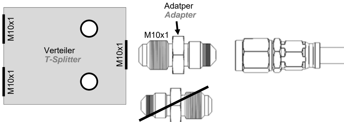
Montageposition 4 / Assembly position 4
