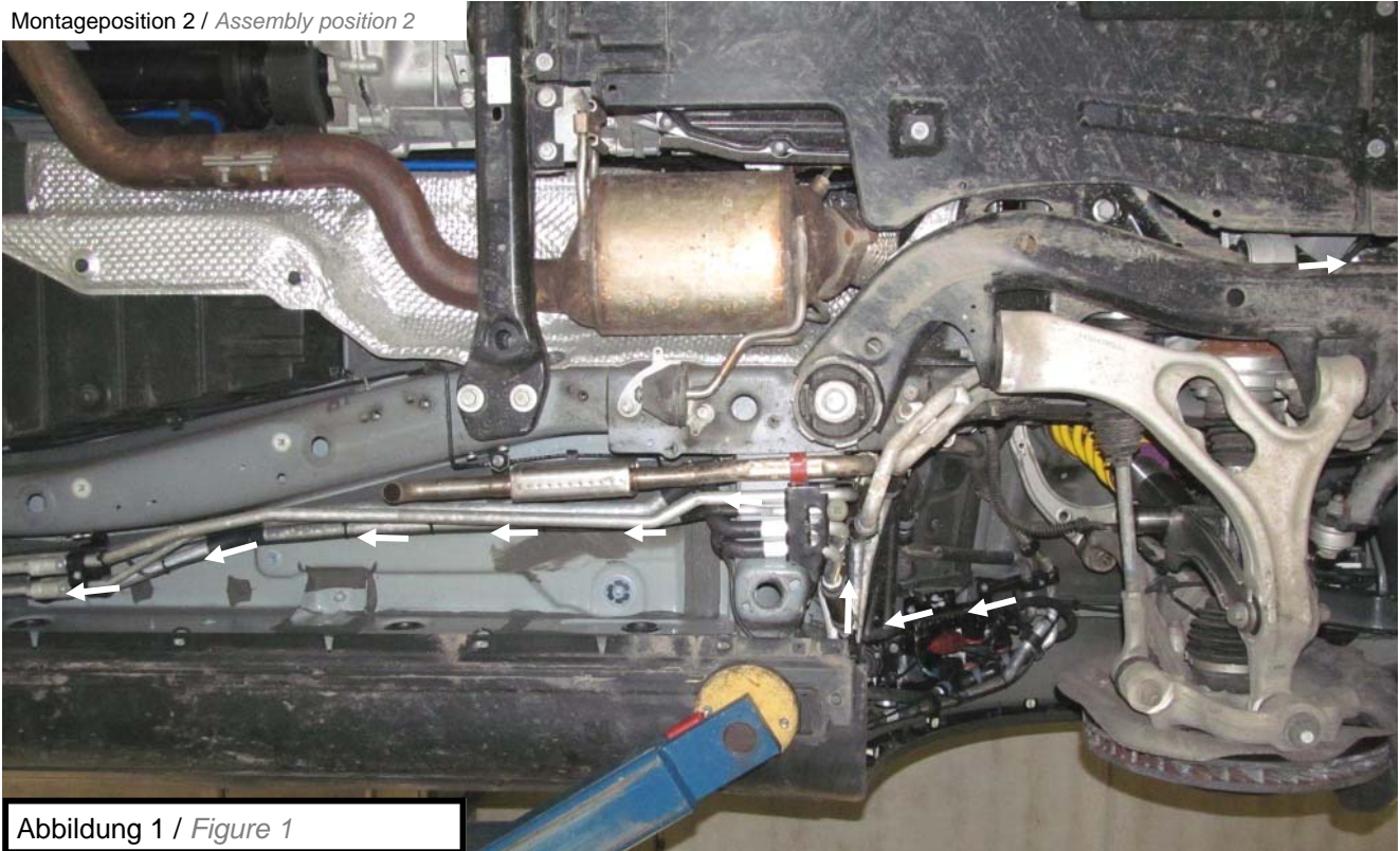
Montageposition 2 / Assembly position 2
