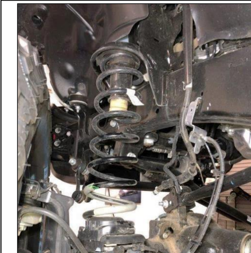
Figure 8: Driver Side shocks removed
