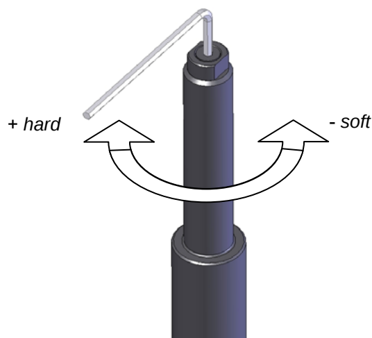
Front axle top
