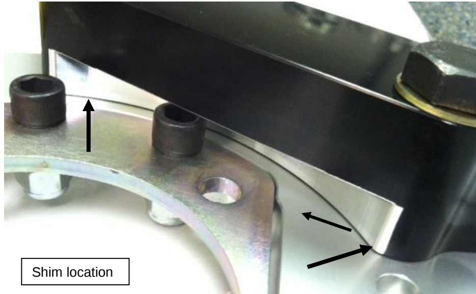
Shims will be placed between the Banksia Plate and the intermediate bracket
